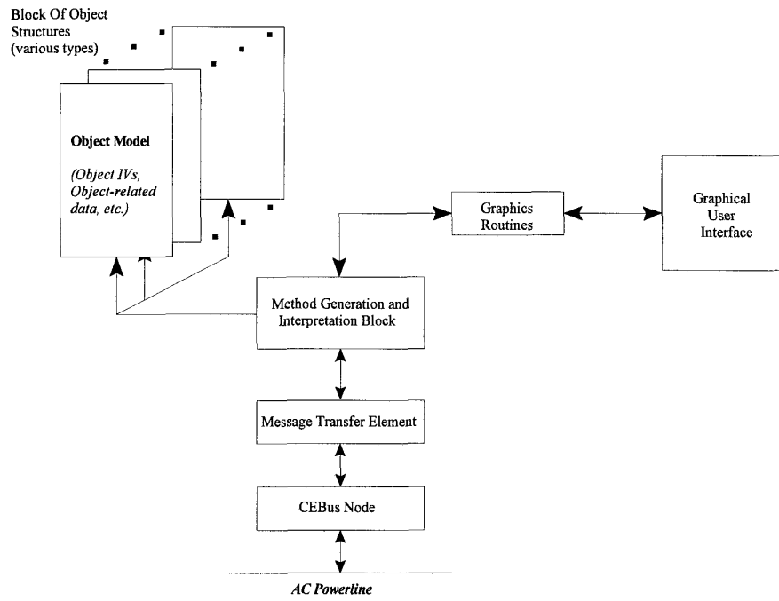
Figure 3: Software structure for PC-based CEBus GUI implementation
