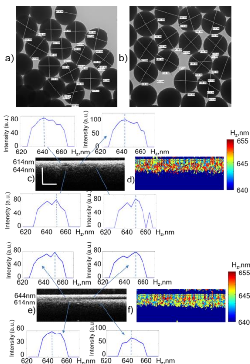
Fig. 1 Images of nanospheres 614 nm and 644 nm diameters; a, b –TEM images c, e - conventional OCT images (B-scans) with axial spatial period profiles for selected locations. d, f, nsOCT images. Lateral and depth scale bars on OCT image are 0.5 mm.
