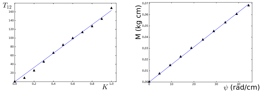
Figure 1: (a) Shear stress response in the simple shear of porcine brain matter; experiments conducted at University College Dublin, see Ref. [3] for details. (b) Torsion of a right cylinder of rubber with radius a = 1.27 cm; digitized data from Ref. [2]. The straight lines represent linear fittings, indicating that the shear modulus is \mu = 163 Pa for brain and 38.2 kPa for rubber.
