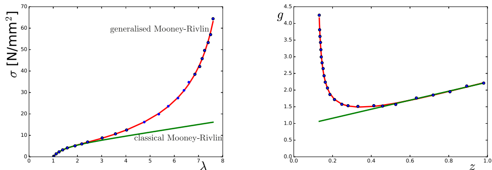
Figure 2: (a) Curve-fitting to Treloar's uni-axial data [7] (circles); Fitted \lambda - \sigma curve the first seven points of the data using the Mooney-Rivlin model (lower curve) and all the data using model W_{\text{gMR}} (upper curve). (b) Mooney plots for the same models and data.
