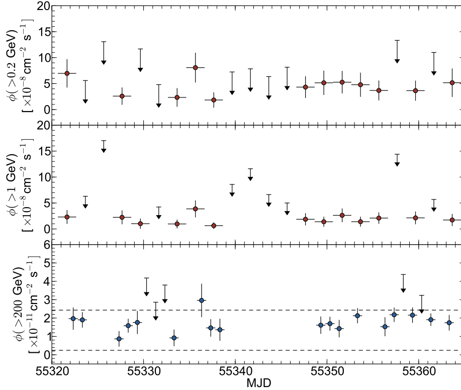
Fig. 3.— Fermi -LAT PG 1553+113 bi-daily flux light curve (2010) above 200 MeV (upper plot) and above 1 GeV (middle plot), in units of \text{cm}^{-2}\text{s}^{-1} , for the time periods contemporaneous with VERITAS observations and VERITAS daily integral flux light curve above 200 GeV (lower plot), in units of \text{cm}^{-2}\text{s}^{-1} (note, for space reasons we do not use notation of \text{ph cm}^{-2}\text{s}^{-1} ). The upper and lower dashed lines indicate the integral fluxes above 200 GeV corresponding to 10% and 1% of the Crab Nebula flux, respectively. The black arrows in all light curves represent 2\sigma upper limits.
