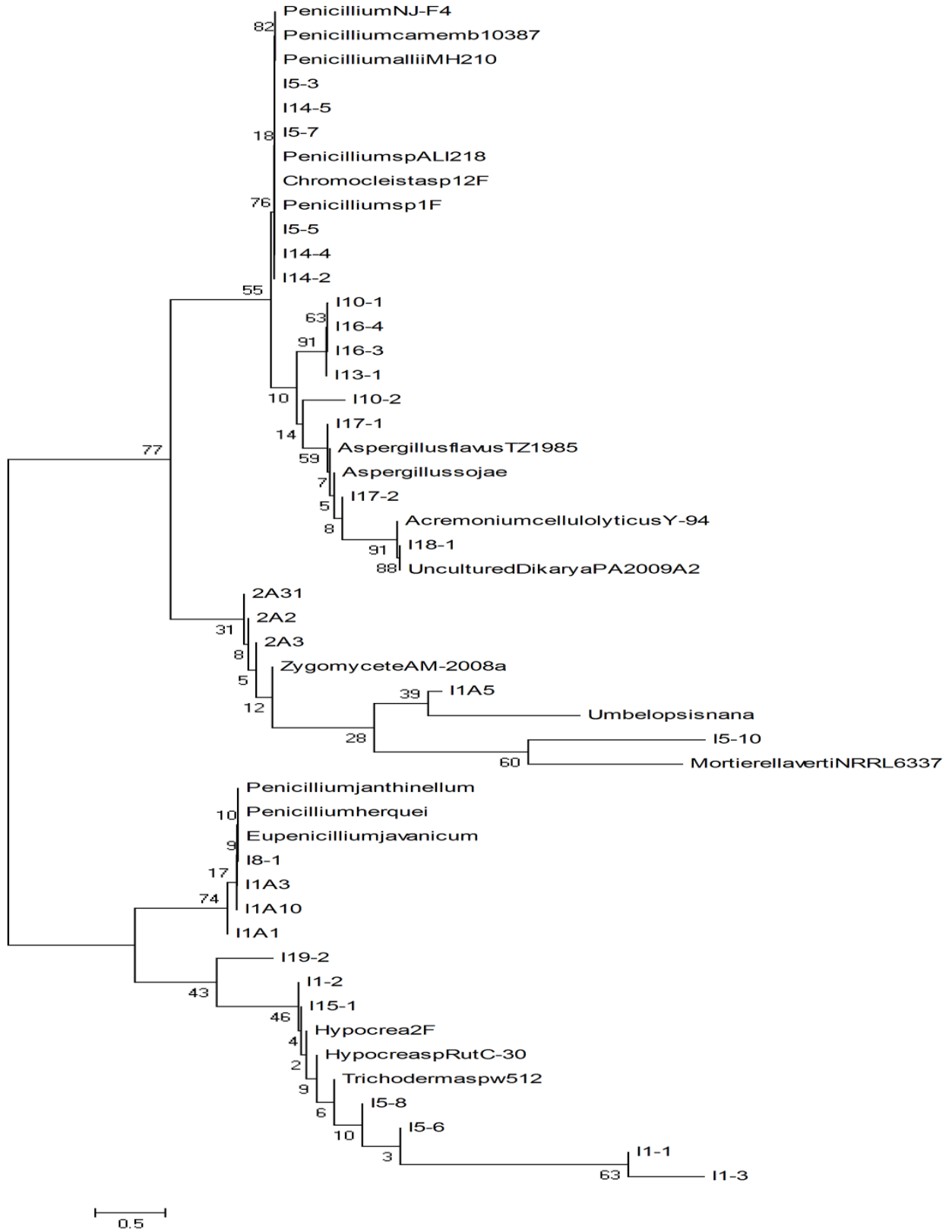
Figure 3.3 Phylogenetic analysis of 18s rDNA of isolated oleaginous fungi
