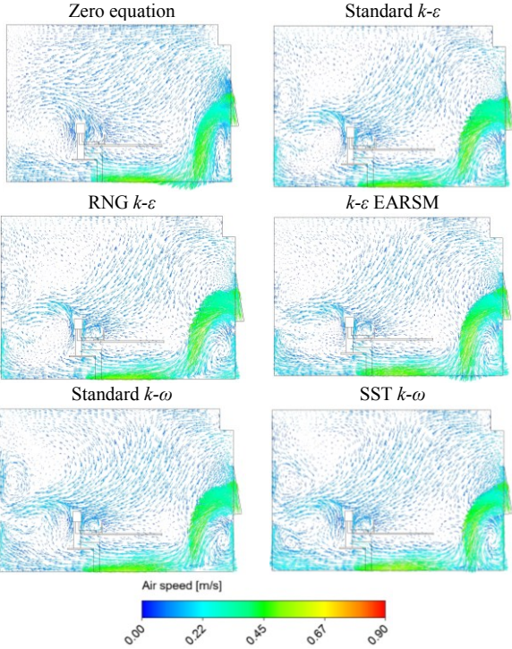
Fig. 4 Airflow distribution inside the room
