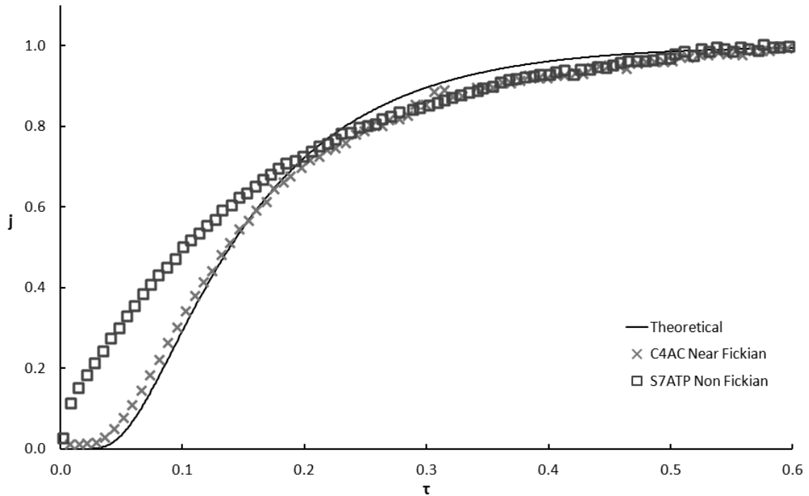
Fig. 3 The non-dimensional leak rate j plotted against non-dimensional time and thickness \tau for (i) theoretical Fickian behaviour, (ii) a near-Fickian Cytec AS4 autoclaved sample and (iii) a non-Fickian Suprem IM7ATP sample.
