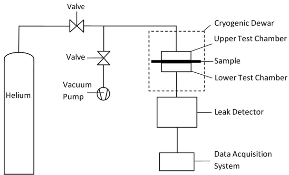
Fig. 1 Schematic of test setup used for leakage testing of laminates showing the helium gas supply, test chamber, cryogenic dewar, leak detector and the data acquisition system.
