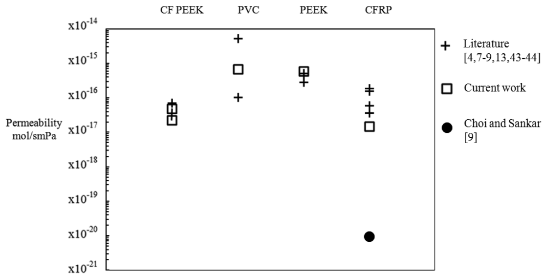
Fig. 4 Comparison of the permeability results from the current work with results reported in literature for CF-PEEK, PVC, un-reinforced PEEK, and CF-Epoxy. The minimum and maximum values for CF-PEEK from the current work are presented [4, 7-9, 13, 43-44].
