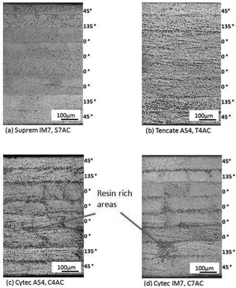
Fig. 2 Micrographs of laminates S7AC, T4AC, C4AC, and C7AC showing the layup and microstructure of each CF-PEEK material.
