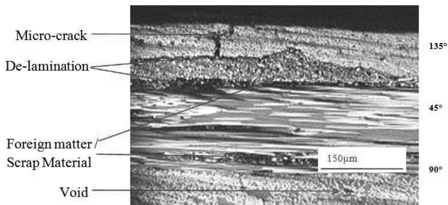
Fig. 6 Micrograph of laminate S7ATP showing a micro-crack, a large de-lamination, a void and scrap material.
