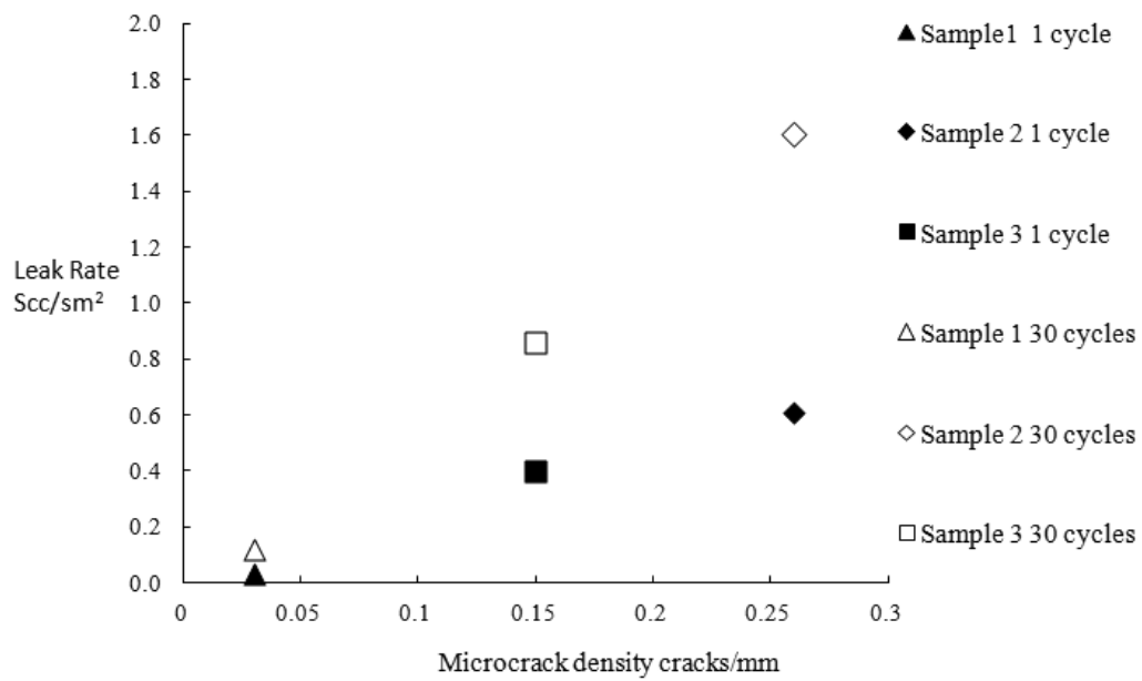
Fig. 10 Leak rate of laminate S7AC1 samples S1, S2 and S3 after cryogenic cycling showing the correlation between measured micro-crack density and leak rate.
