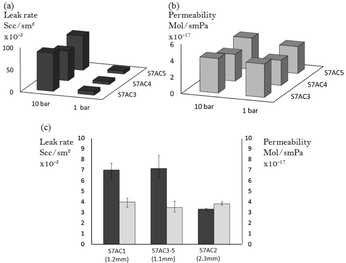
Fig. 5 (a) Leak rate of three samples tested at pressure differences of 1 bar and 10 bar, which shows that the leak rate increases with increasing pressure. (b) Permeability of three samples tested at a pressure difference of 1 bar and 10 bar, which shows that the permeability remains constant at different pressures in line with Fick's law. (c) Leak rate and permeability of samples of different thickness, which shows that leak rate decreases with increasing sample thickness, but the permeability remains constant, in line with Fick's law.
