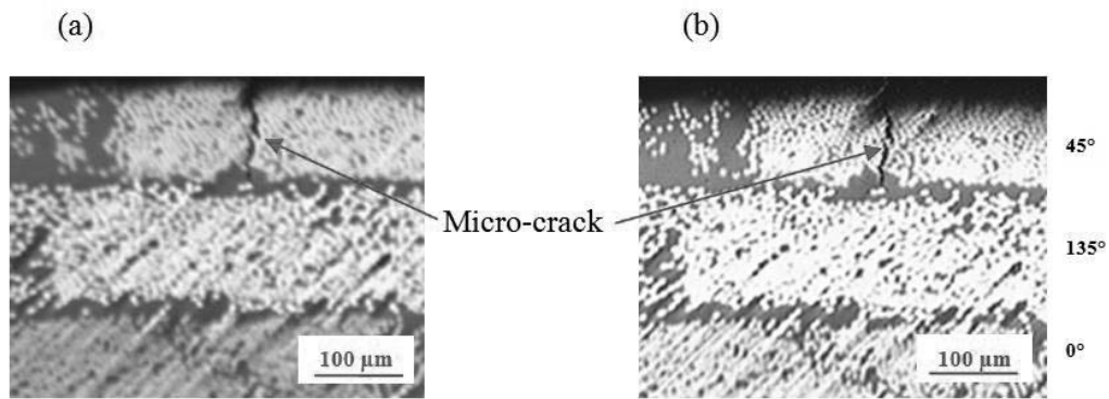
Fig. 7 (a) Micrograph of laminate C4AC showing micro-crack on surface ply before cryogenic cycling. (b) Micrograph showing the same micro-crack after 30 cryogenic cycles.
