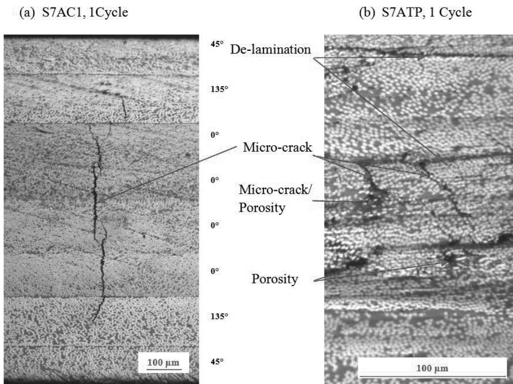
Fig. 8 (a) Micrograph of laminate S7AC1 following one cryogenic cycle, showing a large micro-crack, which propagates through the all four 0° plies and into the 135° plies. (b) Micrograph of laminate S7ATP following one cryogenic cycle which shows de-laminations, micro-cracking, and porosity.
