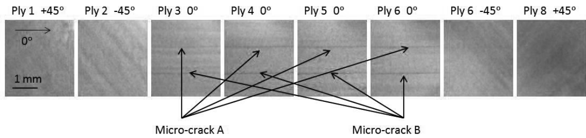
Fig. 9 CT scan of laminate S7AC1 showing ply-by-ply sections of the laminate and micro-cracks A and B in the central plies.
