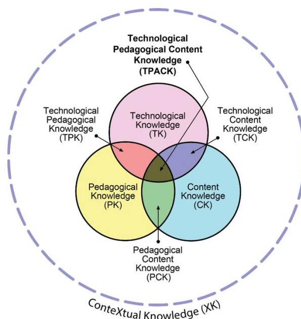
Figure 1. TPACK model [51].
