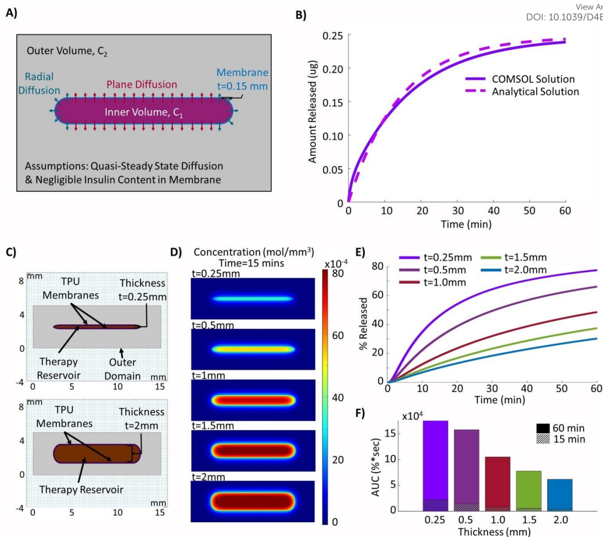
Figure 3: Impacts of changing internal therapy reservoir thickness. A) Diagram depicting set-up for quasi-steady state analytical solution for a device with internal therapy reservoir thickness of 0.5 mm and no flow. B) Comparison of analytical and computational model outputs. Computational model altered to have uniform concentration inside and outside of the therapy reservoir to mimic analytical assumptions. C) Model geometry used in simulation, the top image shows the thinnest device investigated (0.25 mm) and the bottom shows the thickest device investigated (2 mm). Internal therapy reservoir volume is shown in red with membranes in purple. D) Model concentration outputs after 15 minutes for devices of varied internal thickness. E) Insulin release from the devices over a 60 minute period. F) Model area under the curve (AUC) outputs for devices of varied internal thickness at the 15 and 60 minute time points.
