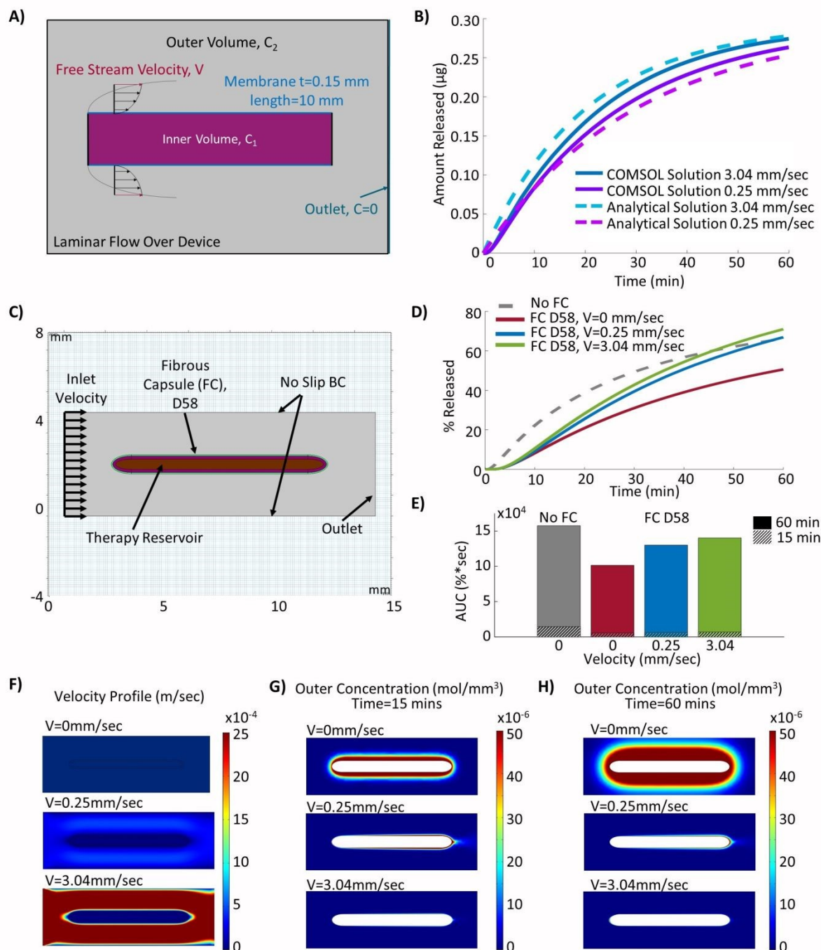
Figure 5: Counteracting the FBR with idealized continuous fluid flow. A) Diagram depicting set-up for analytical verification based on diffusion through a plate subject to transverse laminar flow. B) Comparison of analytical and computational model outputs. Computational model altered to have uniform concentration inside of therapy reservoir to mimic analytical assumptions. C) Model geometry used to build the device with surrounding fibrous capsule (FC) and idealized local fluid flow over the device. D) Insulin release from the device over a 60 minute period. E) Insulin release area under the curve (AUC) at the 15 and 60 minute time points. F) Velocity profile for local fluid flow over the device with inlet velocities of 0 mm/sec, 0.25 mm/sec and 3.04 mm/sec. G) Concentration profiles of the outside of the device after 15 minutes with inlet velocity set to 0 mm/sec, 0.25 mm/sec and 3.04 mm/sec. H) Concentration profiles of the outside of the device after 60 minutes with inlet velocity set to 0 mm/sec, 0.25 mm/sec and 3.04 mm/sec.
