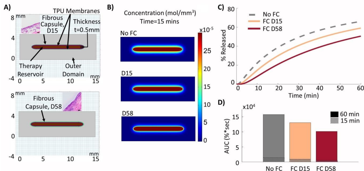
Figure 4: Impacts of the fibrous capsule at various time points. A) Model geometry used to build the device with surrounding fibrous capsule. B) Concentration in model after 15 minutes with no fibrous capsule, and capsule modelled at days 15 and 58. C) Insulin release from the device over a 60 minute period with fibrous capsule (FC) at various times of implantation. D) Insulin release area under the curve (AUC) at the 15 and 60 minute time points.
