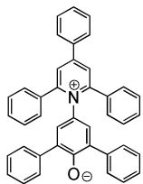
2, 6-diphenyl-4-(2,4,6-triphenylpyridinium-1-yl)phenolate (I)
