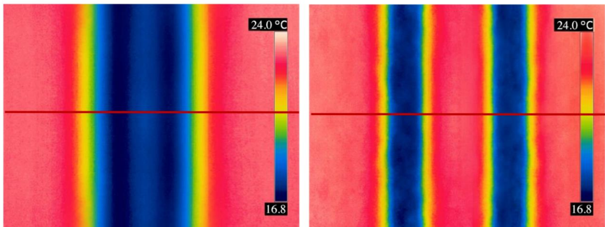
Fig. 4. Sample IR images for Specimen 1 (left) and of Specimen 2 (right).
