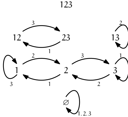
FIGURE 1. \mathcal{S}^* acting on \mathcal{P}(\mathcal{S}) of type A_3 .
