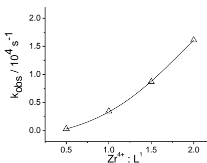
Figure 5. Dependence of the cleavage rate of NPP ( 5 \times 10^{-5} \text{ M} ) on the metal to ligand ratio at \text{pH } 7.0 and 25^\circ\text{C} ; [\text{L}^1] = 1 \text{ mM} ; \text{pH} = 7.0 ; [\text{buffer}] = 50 \text{ mM} (HEPES); I = 0.1 \text{ M} (NaCl).
