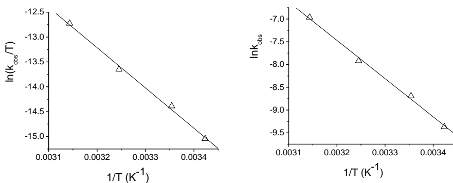
Figure 8. Eyring (left) and Arrhenius (right) plots for the hydrolysis of NPP ( 5 \times 10^{-5} M) by 1 (2 mM) at 25°C and pH 7; [buffer] = 50 mM (HEPES); I = 0.1 M (NaCl).
