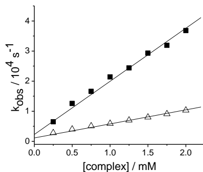
Figure 3. Dependence of the cleavage rate of NPP ( 5 \times 10^{-5} \text{ M} ) on the concentration of 1 ( \Delta ) and 2:1 mixtures of \text{Zr}^{4+} and \text{L}^2 ( \blacksquare ) at 25^\circ\text{C} and \text{pH } 7.0 ; [\text{buffer}] = 50 \text{ mM} (HEPES); I = 0.1 \text{ M} (NaCl).
