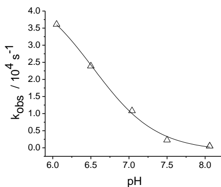
Figure 2. Rate-pH profile of the hydrolysis of NPP ( 5 \times 10^{-5} \text{ M} ) in the presence of 1 (2 mM) in 50 mM buffer at 25 °C. I = 0.1 \text{ M} (NaCl).
