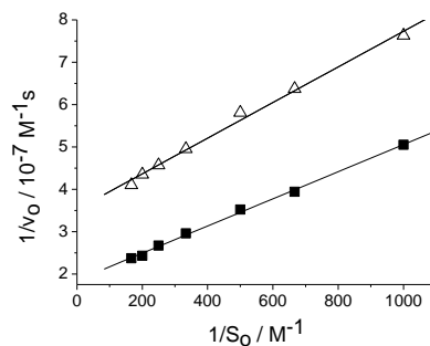
Figure 4. Lineweaver-Burk plots for the hydrolysis of NPP by 1 ( 1.0 \text{ mM} ) ( \Delta ) and 2:1 mixtures of \text{Zr}^{4+} and \text{L}^2 ( 0.5 \text{ mM} ) ( \blacksquare ); 25^\circ\text{C} ; \text{pH } 7 ; [\text{buffer}] = 50 \text{ mM} (HEPES); I = 0.1 \text{ M} (NaCl).
