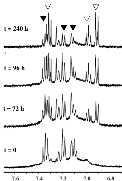
Figure 7. Aromatic region of the ^1\text{H} NMR spectra of phenyl phosphate (10 mM) in the presence of \text{L}^3 (10 mM) and \text{Zr}^{4+} (20 mM) at pD 7.0 and 40 °C. ▼ = phenyl phosphate; ▽ = hydrolysis product
