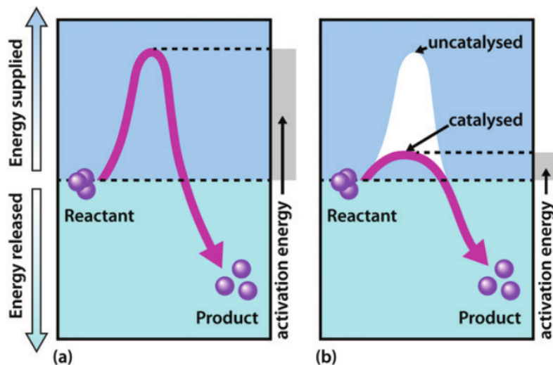
Figure 1.2: An enzyme reduces the activation energy required to initiate a chemical reaction. (a) represents an uncatalysed reaction, and (b) represents an enzyme-catalysed reaction. Extracted from [3].
