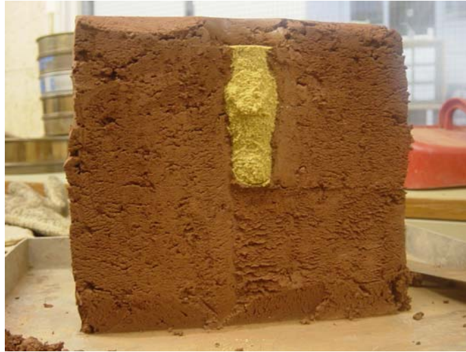
Figure 4: Model tests on stone column showing characteristic bulging behaviour (Plymouth University)
