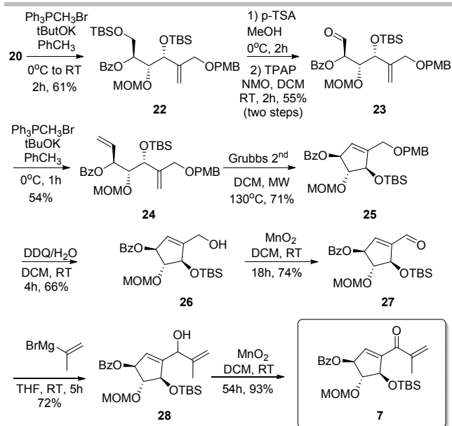
Scheme 3. Synthesis of polyhydroxylated cyclopentene 7 .
