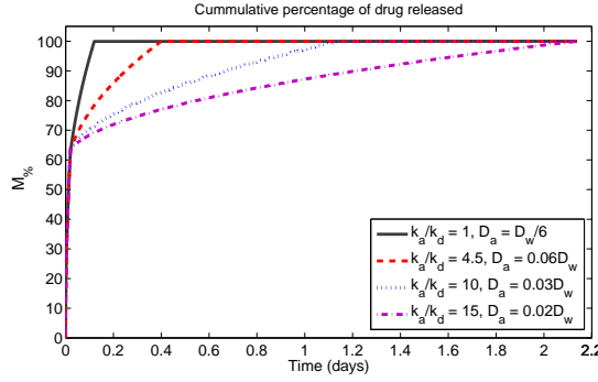
Figure 8: Plot of the cumulative fraction of drug released from a two-stage release system for various D_a/D_w corresponding to varying the ratio k_a/k_d . Here we plot the numerical solution for the default parameter values in Table 1 except that L_p = 5 \times 10^{-5} m and L_d = 10^{-4} m.
