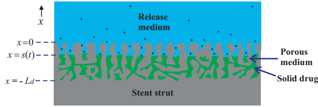
Figure 3: A diagram introducing some of the notation used. Here x = 0 locates the interface between the porous medium and the release medium, and the boundary x = s(t) gives the position of a moving dissolution front separating the undissolved and dissolved drug.
