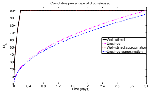
Figure 9: A comparison between the cumulative percentage of drug released ( M\% ) from the nanoporous system in unstirred and well-stirred release media. Also on display are the approximate solutions for the case of poorly soluble drugs. In each case we have c_s/c_0 = 0.1 < 1 . We observe that drug release is significantly sped up in the well-stirred release medium, as one would expect. Furthermore, the respective approximate solutions for poorly soluble drugs are providing good agreement with the full solutions, even for c_s/c_0 = 0.1 . The agreement improves as c_s/c_0 is reduced further. The default parameter values used in the generation of this plot are displayed in Table 1.
