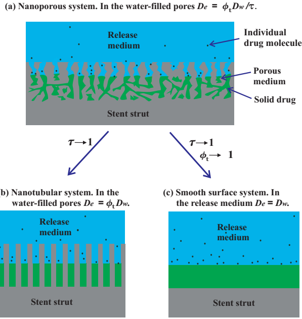
Figure 2: (a) The stent drug delivery system. A drug-infused porous medium overlays the stent strut. In the liquid-filled pores, the drug has diffusivity D_e = \phi_t D_w / \tau , where \phi_t is the effective porosity of the medium and \tau is its tortuosity. (b) Taking the limiting case of the tortuosity tending to one ( \tau \rightarrow 1 ) gives the case of a nanotubular system. (c) Taking the limiting case of \tau, \phi, \phi_t \rightarrow 1 and \phi_s, k_a/k_d \rightarrow 0 gives the case of a pure drug layer with no porous medium.
