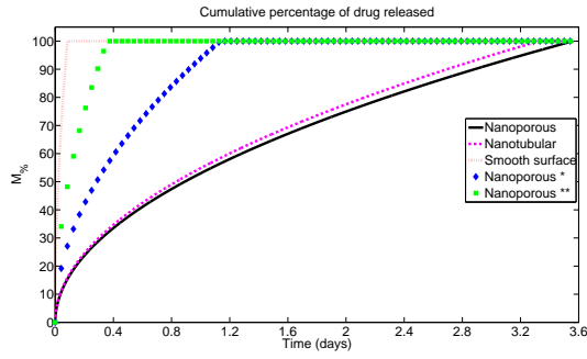
Figure 5: A comparison between the cumulative percentage of drug released ( M\% ) for a nanoporous, nanotubular and smooth surface system. We observe that a nanotubular system results in quicker release of drug than a nanoporous system due to less tortuous pores. The smooth surface system results in a dramatic increase in the rate of drug release, since there are no pores to hinder the release of drug. Two additional cases have been added to demonstrate one way in which the nanoporous system can be tuned to achieve quicker release profiles. Nanoporous* and Nanoporous** have the reduced porosities \phi = \phi_t = 0.3 and \phi = \phi_t = 0.1 , respectively. The default parameter values used in the generation of this plot are displayed in Table 1.
