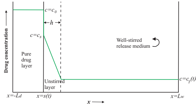
Figure 10: The special case of a pure drug layer in a well-stirred release medium. This case cannot be described by the solution (30), (31) and must be considered separately. A narrow boundary layer of poorly stirred fluid forms near the surface of the solid drug, and it is assumed that the flux of drug from the dissolving surface is proportional to the difference between the drug concentration at the surface and the drug concentration in the well-stirred release medium.
