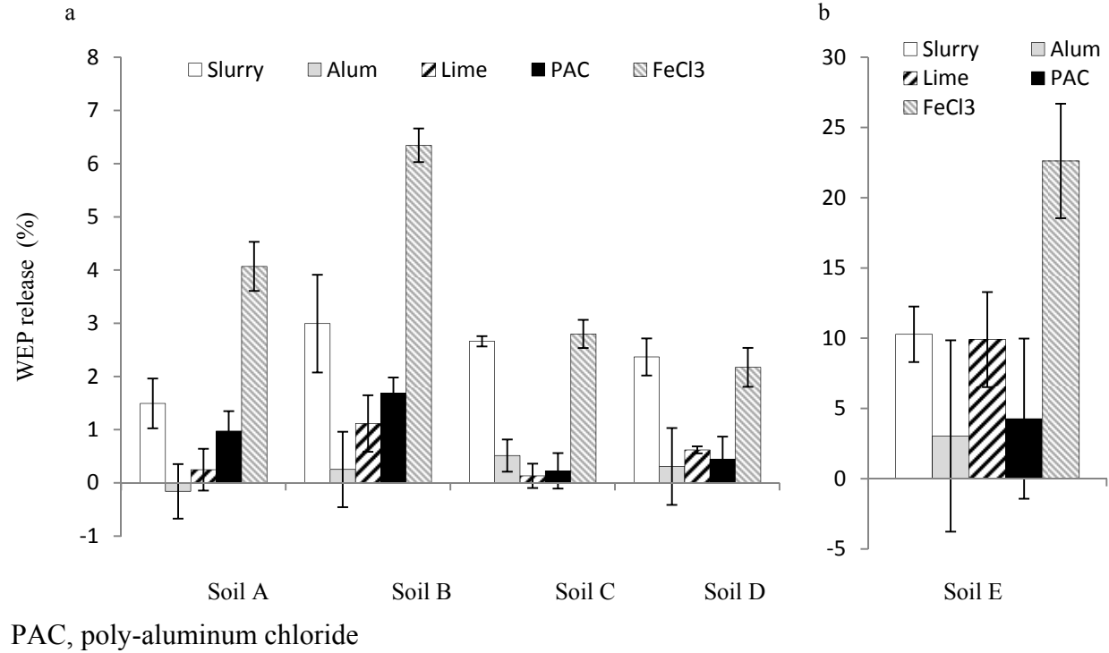
Figure 1. Water extractable phosphorus release (WEP) expressed as a percentage of total phosphorus applied for nine month compared to soil-only treatment (a) the four mineral soils (b) peat soil (PAC, poly-aluminum chloride)
