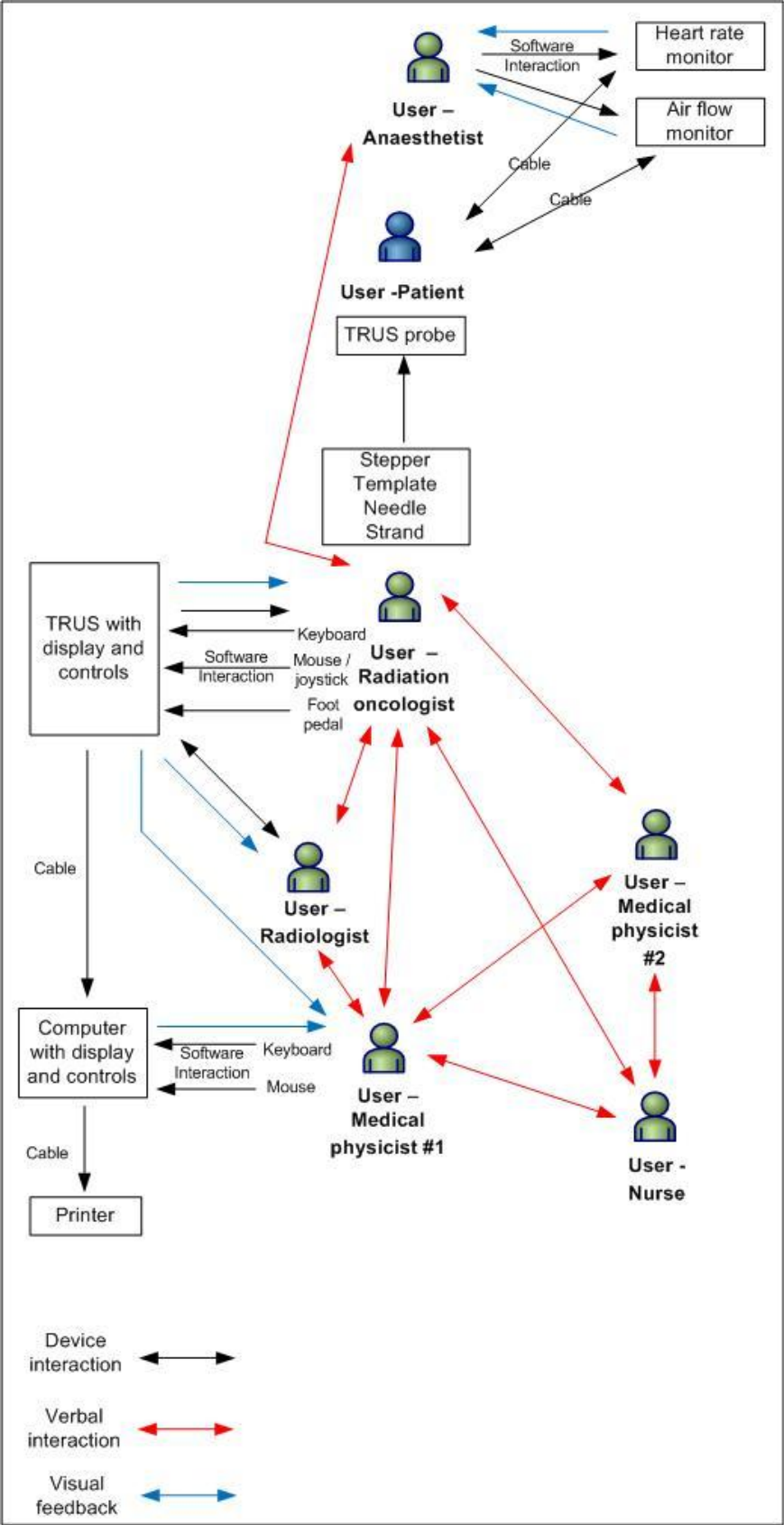
Figure 3-4 User-system interaction diagram of “stranded seeds” LDR prostate brachytherapy setup
