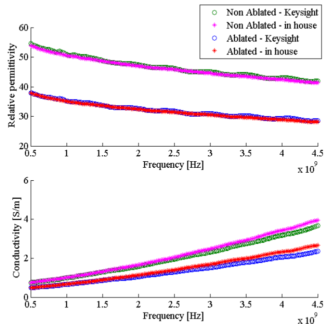
Fig. 2. Comparison of the “Stuchly and Stuchly” method with the Keysight method: dielectric measurements (mean values) as a function of frequency, performed in both ablated and non-ablated ovine liver with a slim-form probe connected to a VNA.
