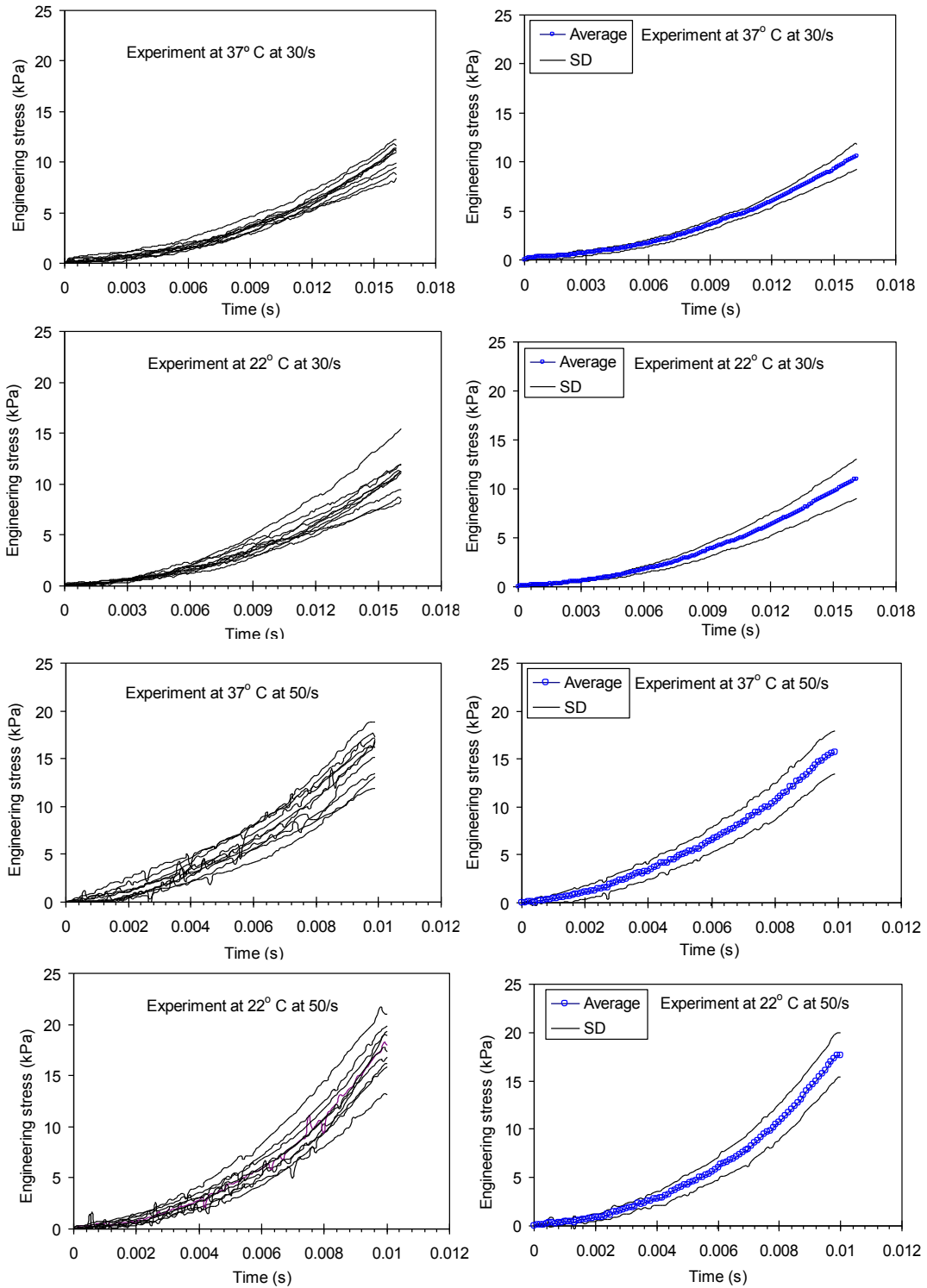
Fig. 2 – Brain tissue behavior at variable loading (30 and 50/s) and temperature conditions (22° C and 37° C)
