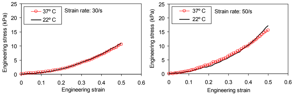
Fig. 3 – Comparison of average engineering stresses.
