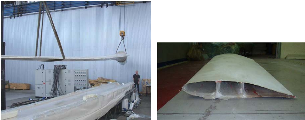
Figure 9. Glass-fibre reinforced PBT thermoplastic wind turbine blade, 12.6 metre length, manufactured at 200°C, (left) removing moulded blade from tool; and (right) a 4.0m moulded section of the blade, showing the spar-cap and shear-webs moulded in a “one-shot” process.
