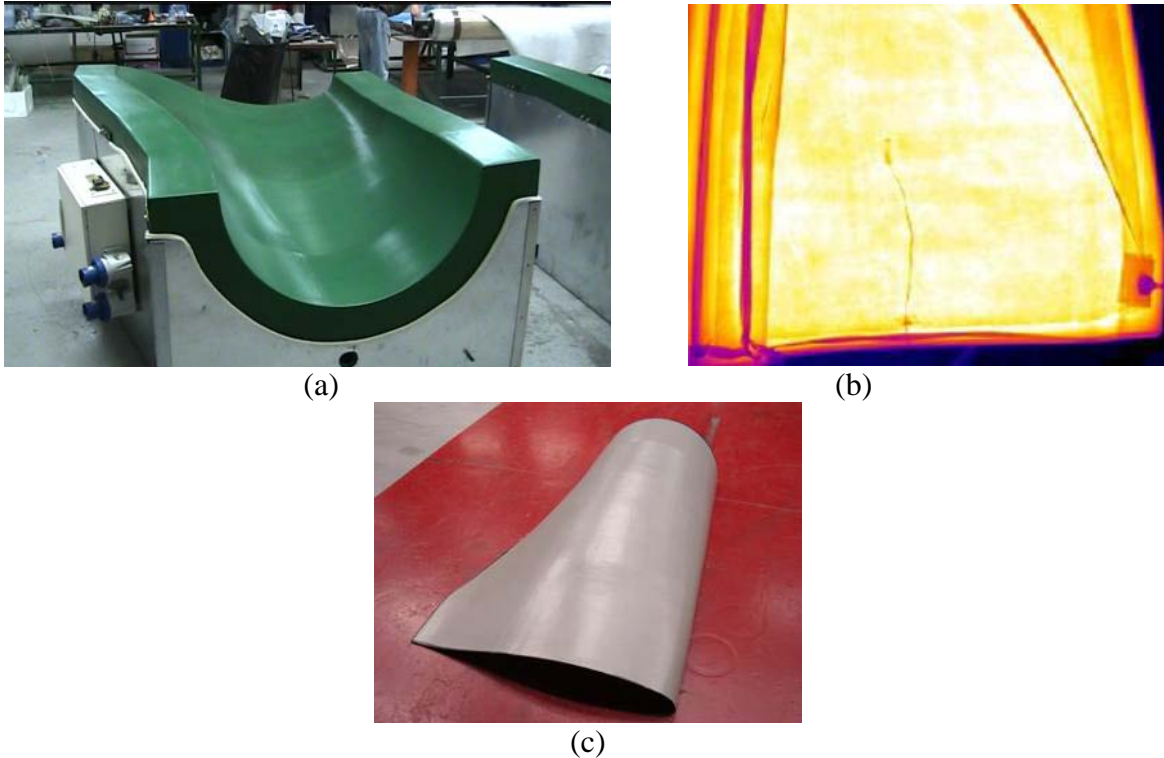
Figure 11. Demonstrator tool (a), measuring 2.0m in length; (b) thermal camera image of temperature in tool with electric heating; and (c) carbon-fibre/epoxy aerospace prepreg part manufactured on tool.
