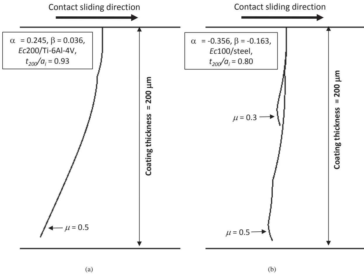
Fig. 9. Predicted effect of COF on coating crack propagation in 200 \mu m thick coating for \alpha values of (a) 0.245, and (b) -0.356 ( P = 500 \text{ N/mm} , \delta = 0.1 \text{ mm} , K_{IC} = 100 \text{ MPa}\cdot\text{mm}^{1/2} ), (Same scale is applied on vertical and horizontal axis).
