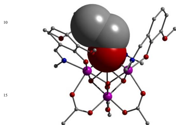
Figure 7 Space-fill representation of the μ 3 -bridging OEt ligand which sits within a molecular cavity forged by the three L 1 ligands in 5 .
