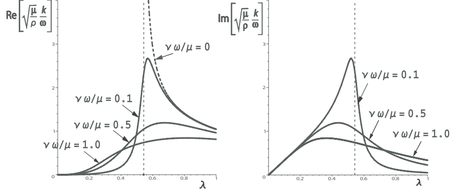
Figure 1: Dimensionless slowness and damping factor for a surface wave with real frequency in a Mooney-Rivlin viscoelastic solid subject to plane strain. The analysis shows that the half-space becomes unstable when compressed by more than about 46% (vertical asymptote) and this confines the validity of the curves to the right of the vertical dashed line.
