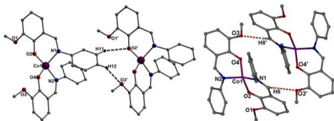
Fig. 7 Crystal structure of [\text{Co}(\text{II})(\text{L}_2)_2] ( 5 ) highlighting the close proximity of neighbouring monomers within the H-bonded chains (left) and between the chains (right). H-bonding shown using dashed lines.
