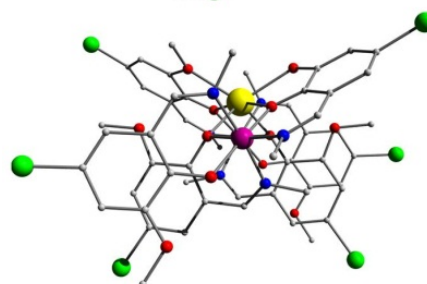
Fig. 8 Crystal structures of [\text{Co}(\text{III})_2\text{Na}(\text{I})(\text{impp-Br})_6](\text{BF}_4) ( 6 ) as viewed perpendicular (top) and parallel (bottom) to the V-shaped plane of the molecule. Colour code: Purple (Co), Yellow (Na), Red (O), Blue (N), Green (Br) and Grey (C). H-atoms omitted for clarity.
