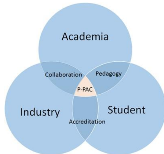
Fig. 1. P-PAC Framework
