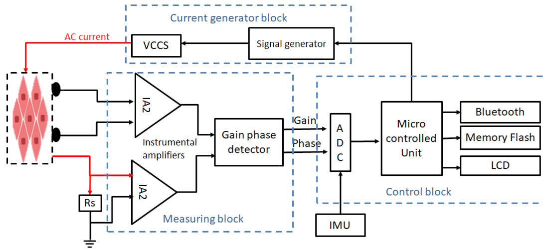
Figure 3: Schematics of the bioimpedance measurement device.
