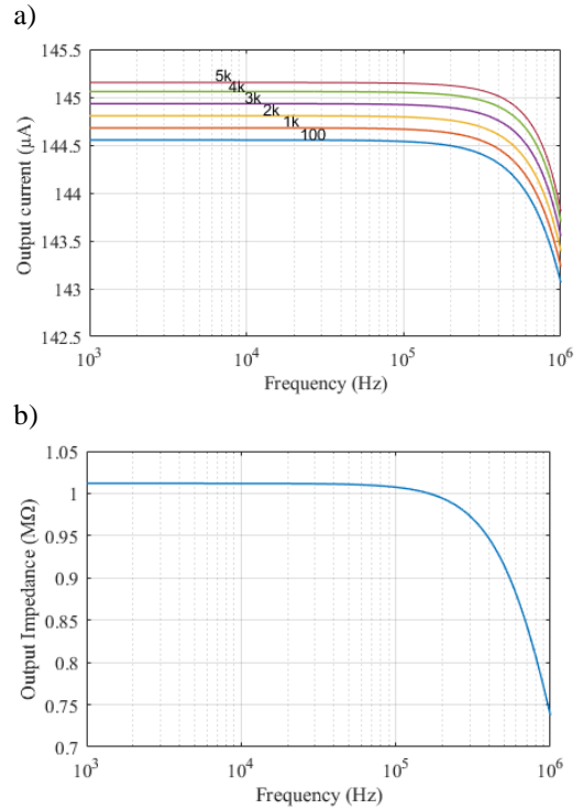
Figure 5: (a) Output current of VCCS for R_L=100 \Omega , 1 \text{ k}\Omega , 2 \text{ k}\Omega , 3 \text{ k}\Omega , 4 \text{ k}\Omega , 5 \text{ k}\Omega . (b) Output impedance of VCCS.
