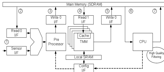
Fig 1: Advanced Hardware Face Detector Block Diagram
