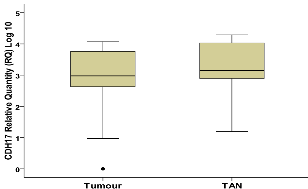
Figure 4.5: CDH17 expressions in CRC. CDH17 expression was significantly lower in colorectal tumours compared to tumour-associated normal tissues ( p < 0.001 )
