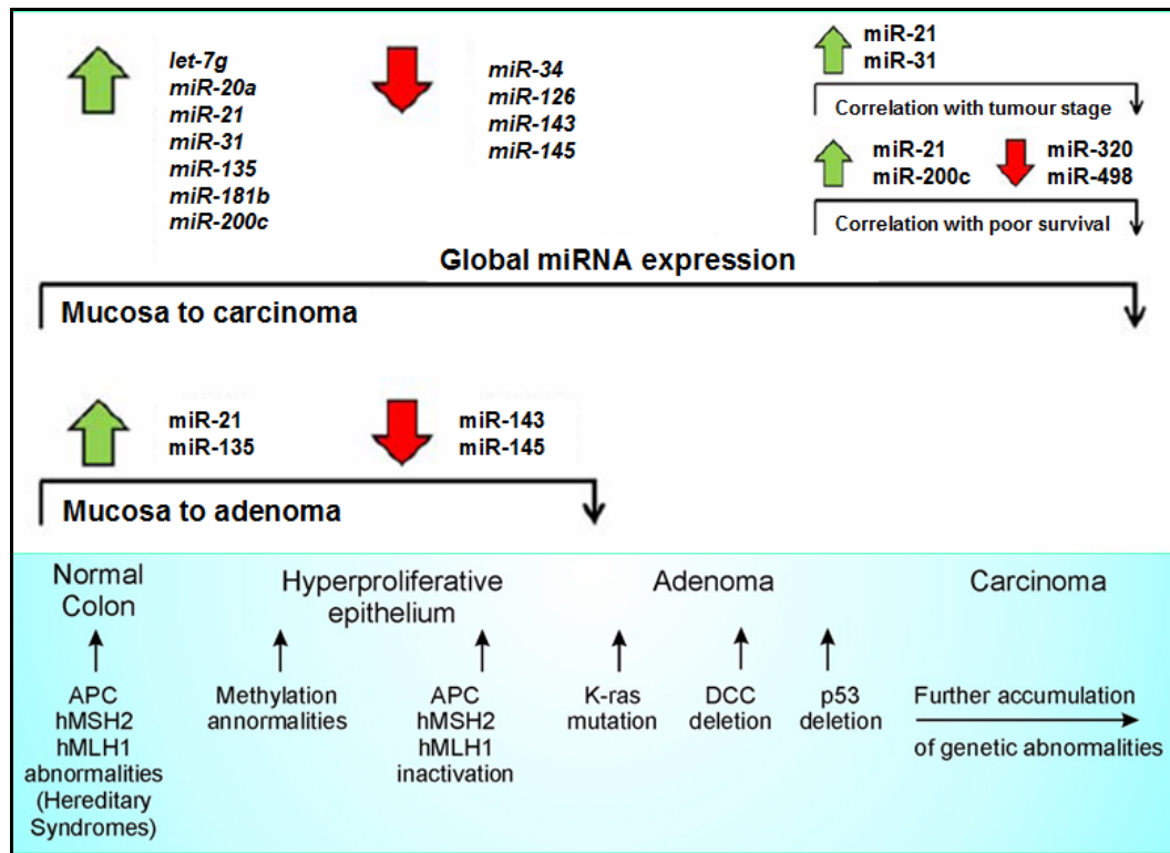
Figure 1.4: miRNA expression in colorectal tumours and their correlations
