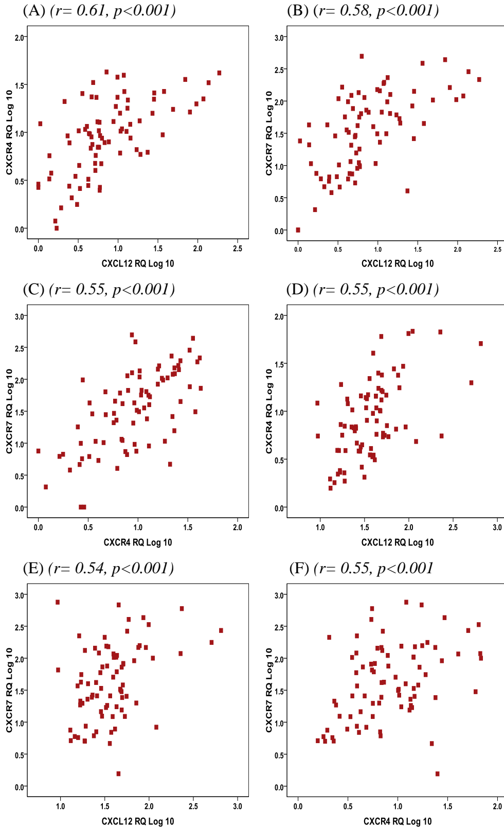
Figure 4.9: Correlations of expression levels of CXCL12 and its receptors Pearson's correlations of expression levels of CXCL12 , CXCR4 and CXCR7 in tumour (A, B, C) and tumour-associated normal (D, E, F) colorectal tissues.
