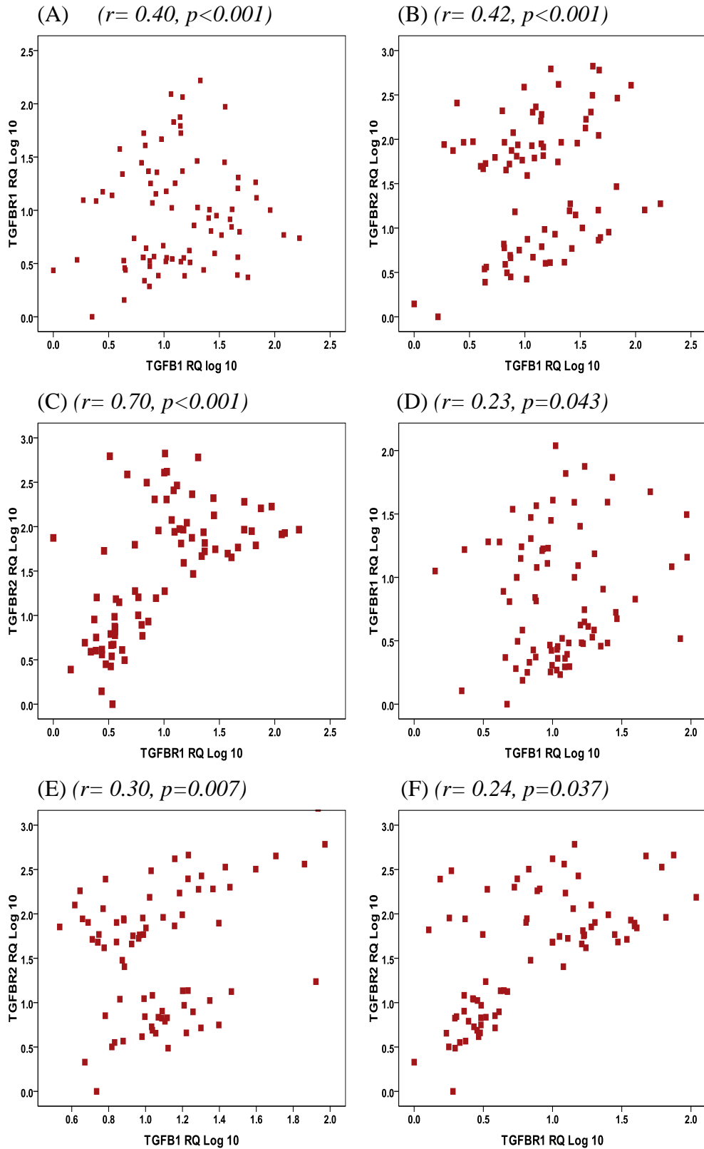
Figure 4.20: Correlations of expression levels of TGFB1 and its receptors Pearson's correlations of expression levels of TGFB1 , TGFB1R1 and TGFB1R2 in tumour (A, B, C) and tumour-associated normal (D, E, F) colorectal tissues.
