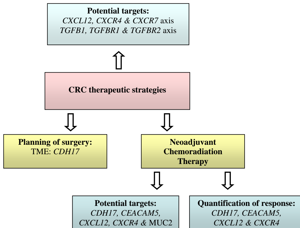
Figure 8.2: Gene expression and CRC management strategies.
