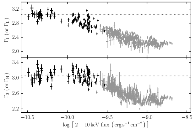
FIG. 6.— Comparison of the spectral trends revealed in our data (black symbols) with the ones published by Giebels et al. (2007) (grey symbols). For this set of fits to the NuSTAR data the break energy ( E_b ) was kept fixed at 7 keV. The uncertainties are given at the 68% confidence level in order to match the previous results. Note the smoothness of the trends covering nearly two orders of magnitude and the apparent saturation effects at each end. The dotted lines are median photon indices for 2–10 keV flux below 10^{-10} erg s ^{-1} cm ^{-2} , representing the apparent low-flux saturation values.
