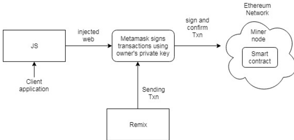
Figure 8. Ethereum transactions workflow
